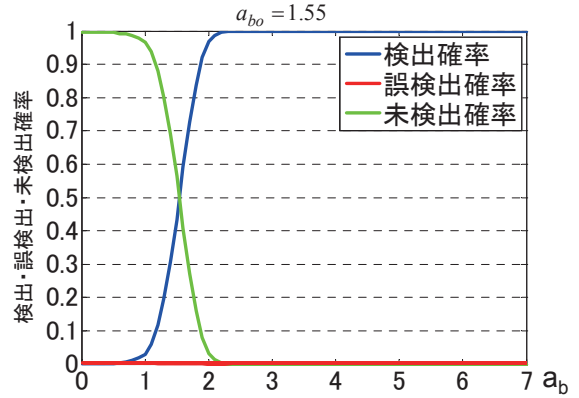
Fig. 25 a_b vs. each probability characteristics ( a_{bo}=1.55 )
