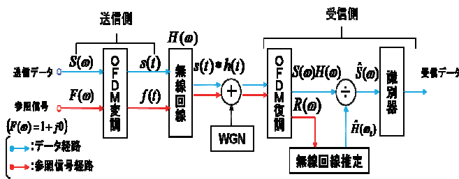
Fig. 3 Structure of transmitter and receiver
