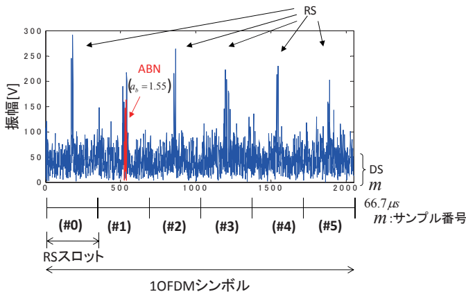
Fig.14 Received signal
