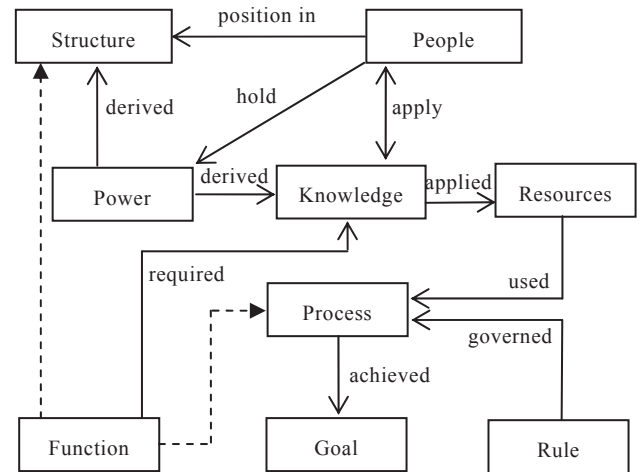
Fig.2 The Knowledge Atlas Schema.
